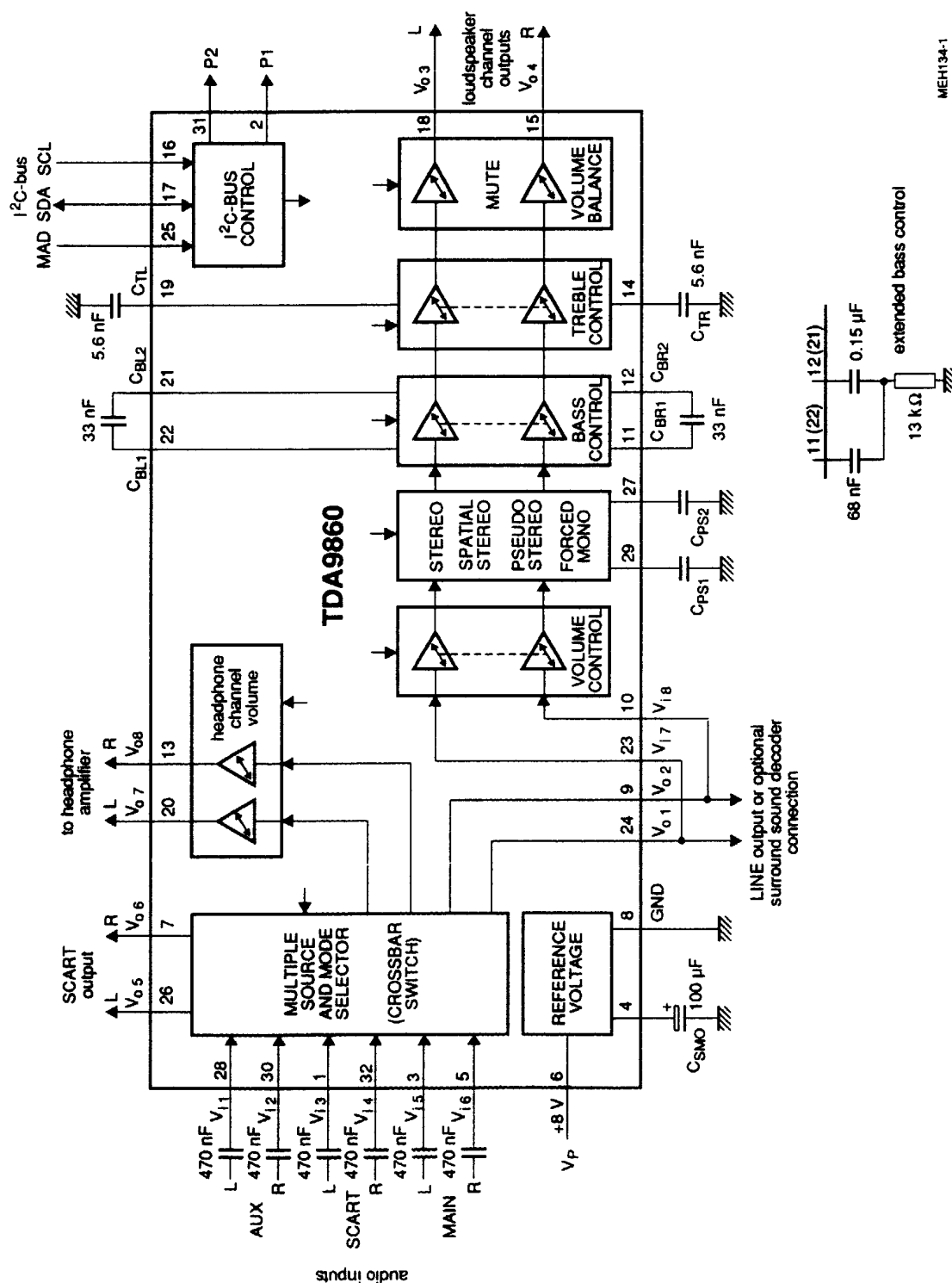
Fig.1 Block diagram and application circuit.
